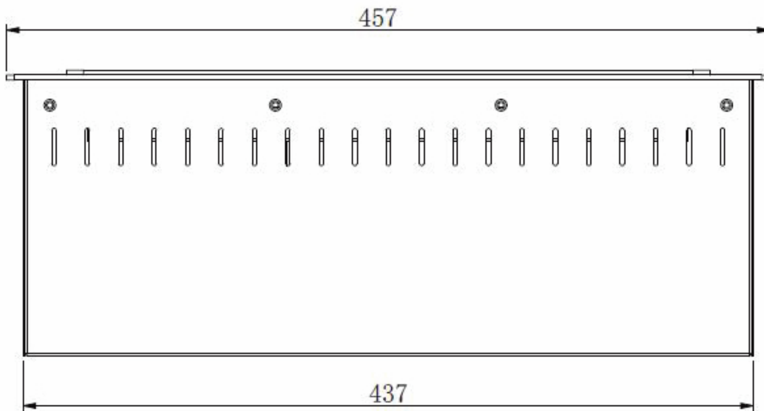
Front View
